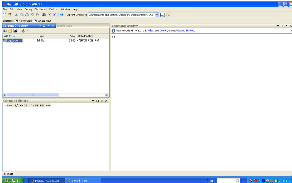
Matlab R2007b
